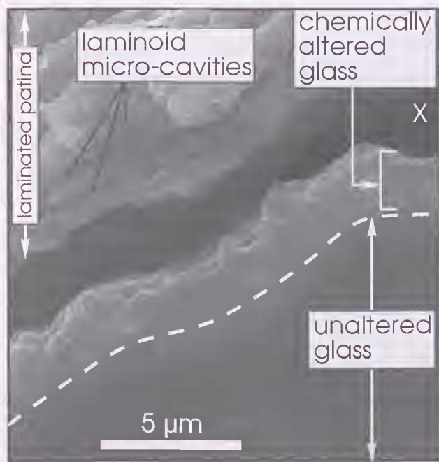
Figure 4. SEM image of a cross-sectional view of patina on glass (sample A1) showing details of features across the glass-to-patina interface. The image also shows a close-up of laminoid micro-cavities within the patina lamination. The black zone (marked X) between the glass and the patina is a separation crack formed during sample preparation.
